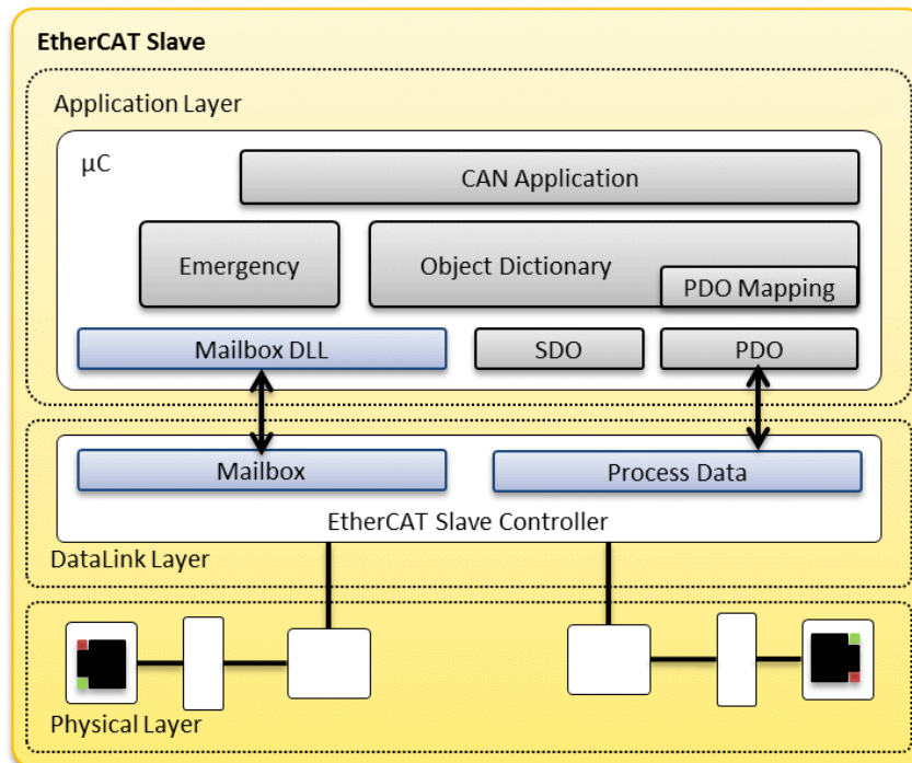
Figure 13: ESC structure for CAN application profile applications
