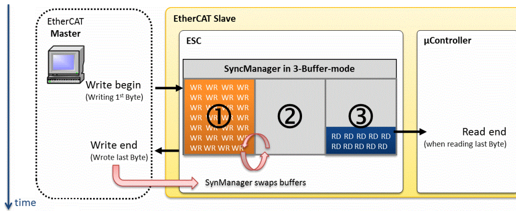
Figure 9: SyncManager 3-buffer-mode
