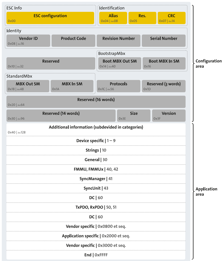
Figure 6: SII layout
