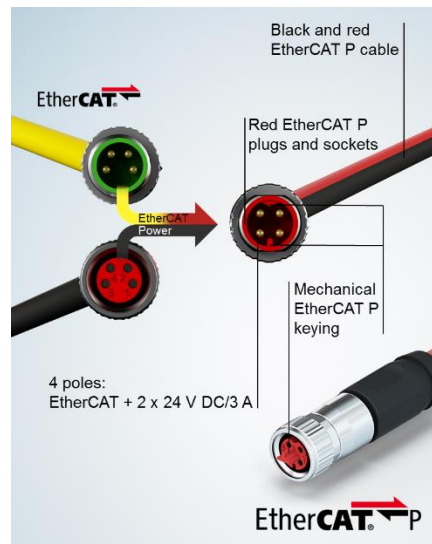
Figure 2: M8 P-coded connector and cable
