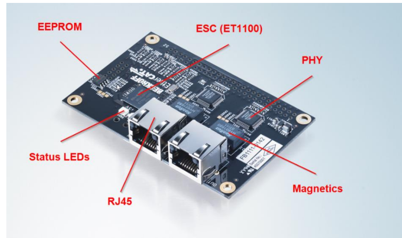
Figure 2: Beckhoff FB1111
